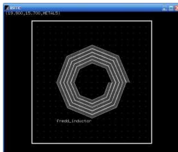
Figure 4. Spiral inductor layout using ASITIC.
