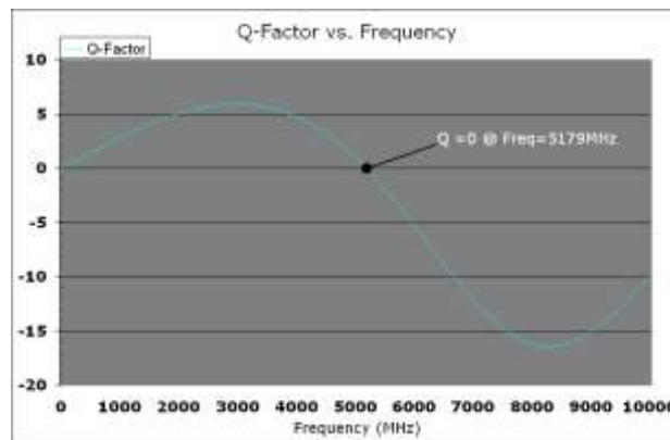
Figure 6. Q-factor plot versus frequency.
