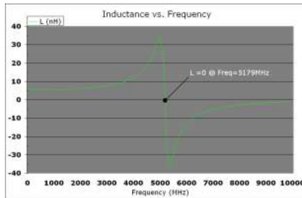
Figure 5. Inductance plot versus frequency.
