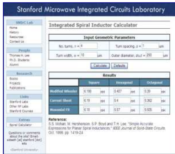
Figure 2. SpiralCalc interface.
