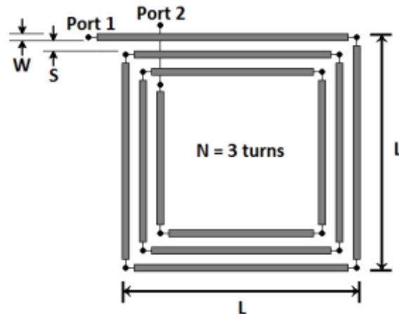
Figure 1. Simplified layout of microstrip spiral inductor.
